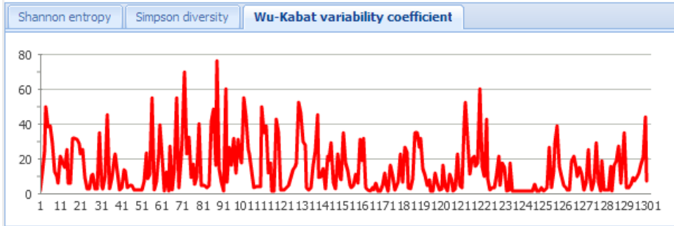
Fig. 6. Wu-Kabat variability by column in a P. falciparum PfEMP1 protein multiple sequence alignment.
